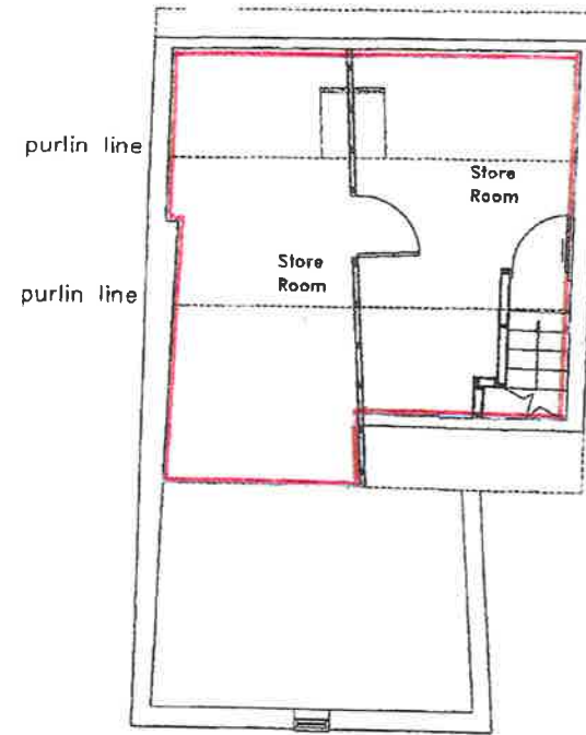
Second Floor Layout
